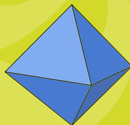
octaedro
