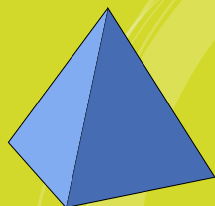
piramide
