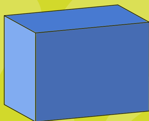
prisma
