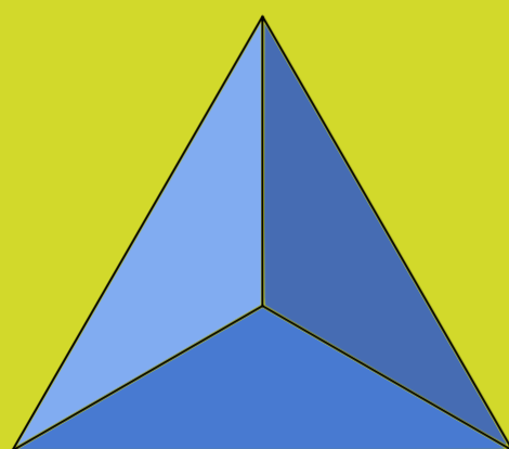
tetraedro
